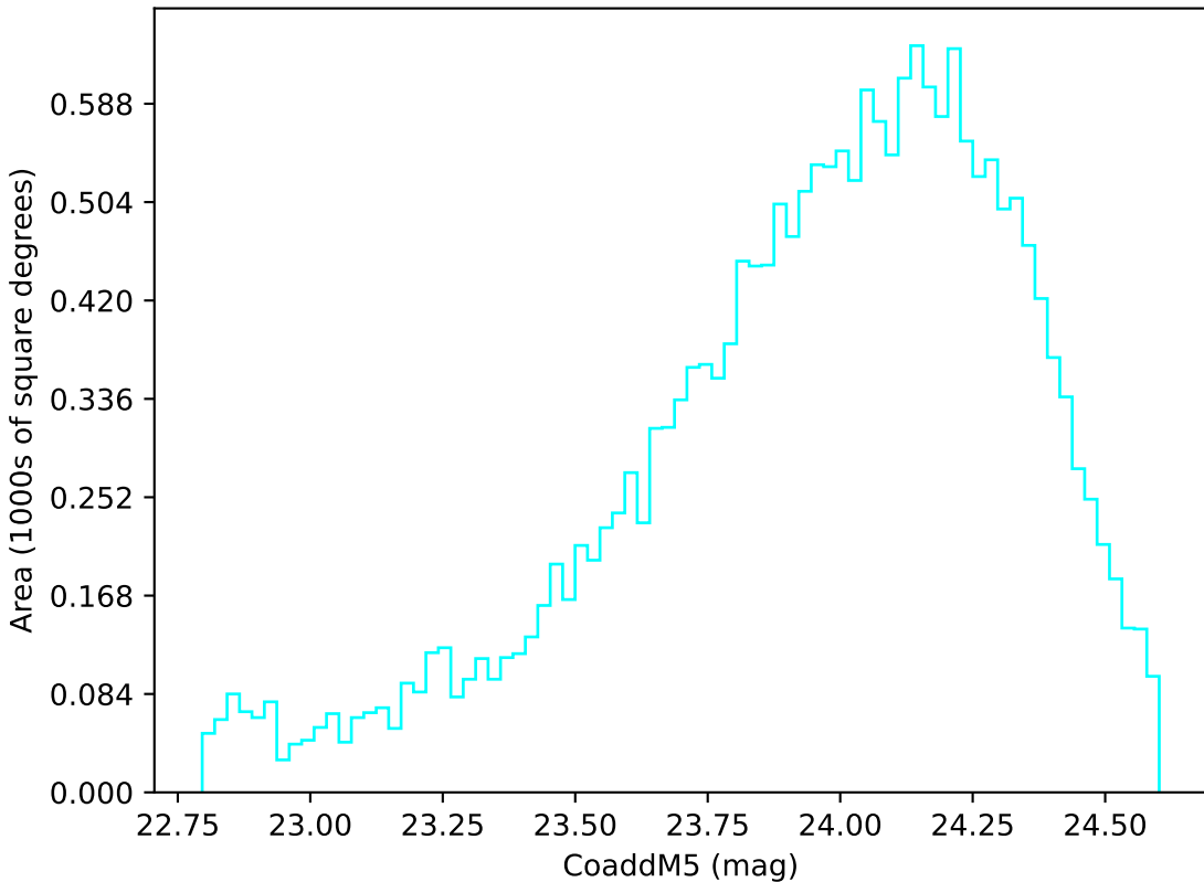
noroll_mjdp180_v3.4_10yrs Yr 3-4 u band: CoaddM5
