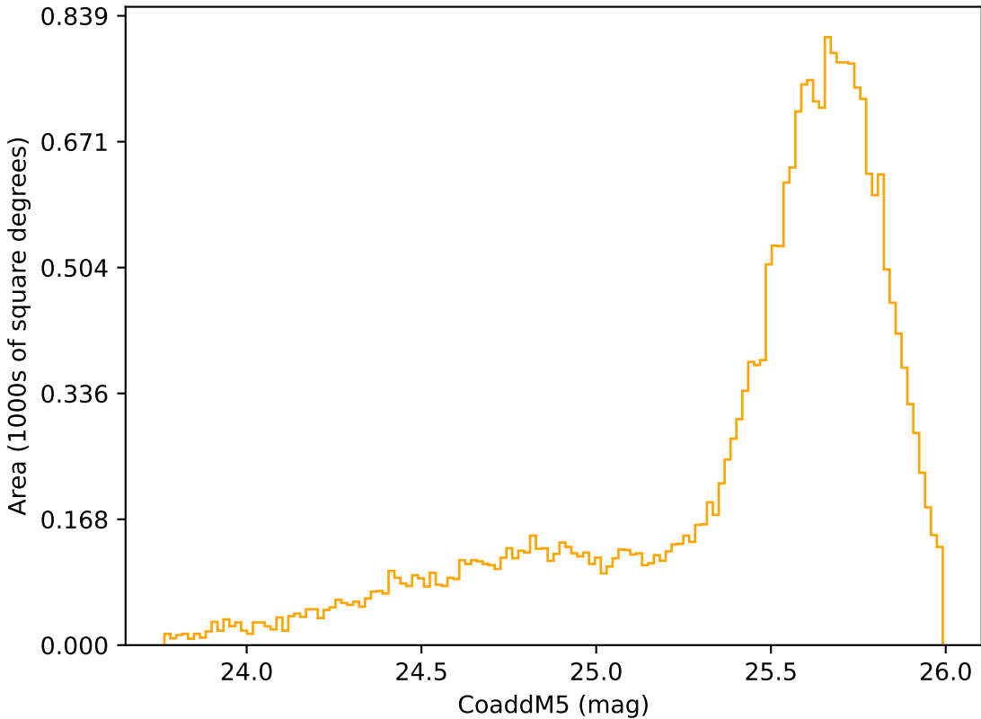
noroll_mjdp180_v3.4_10yrs Yr 3-4 r band: CoaddM5
