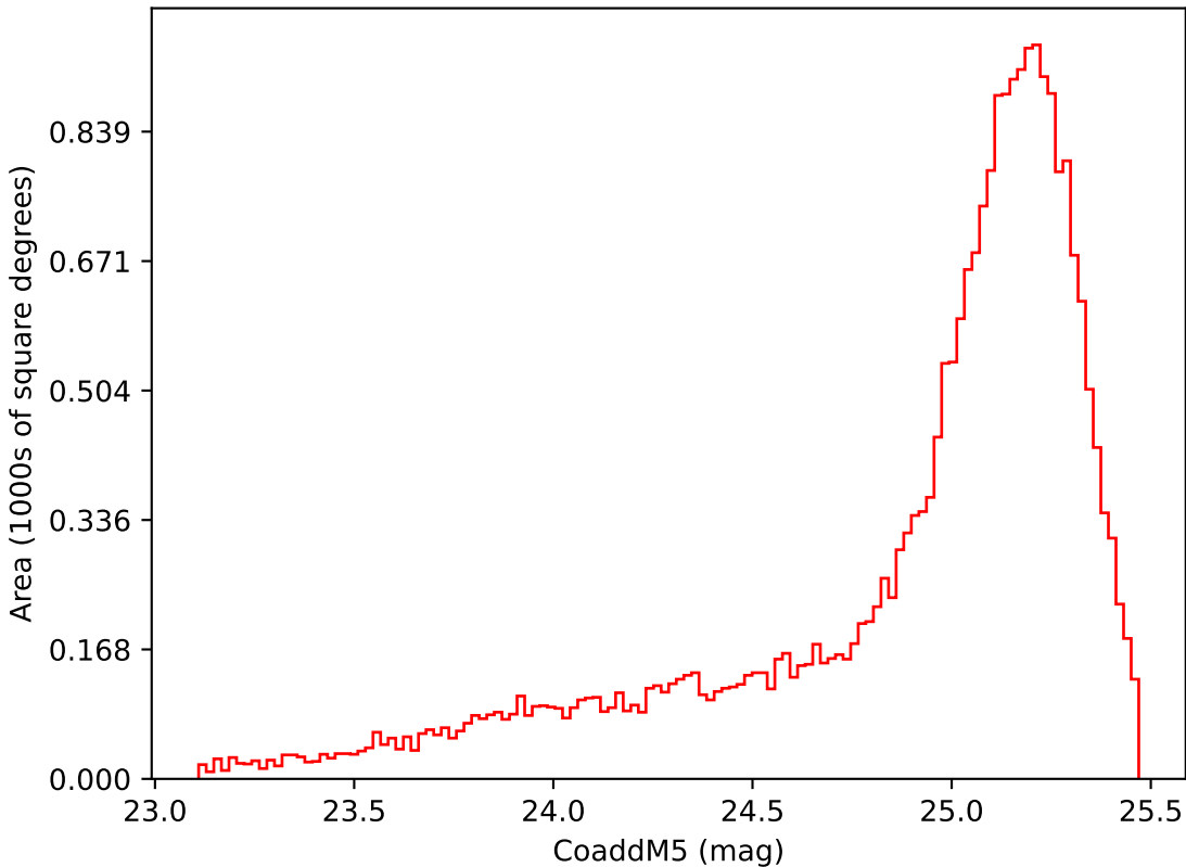
noroll_mjdp180_v3.4_10yrs Yr 3-4 i band: CoaddM5
