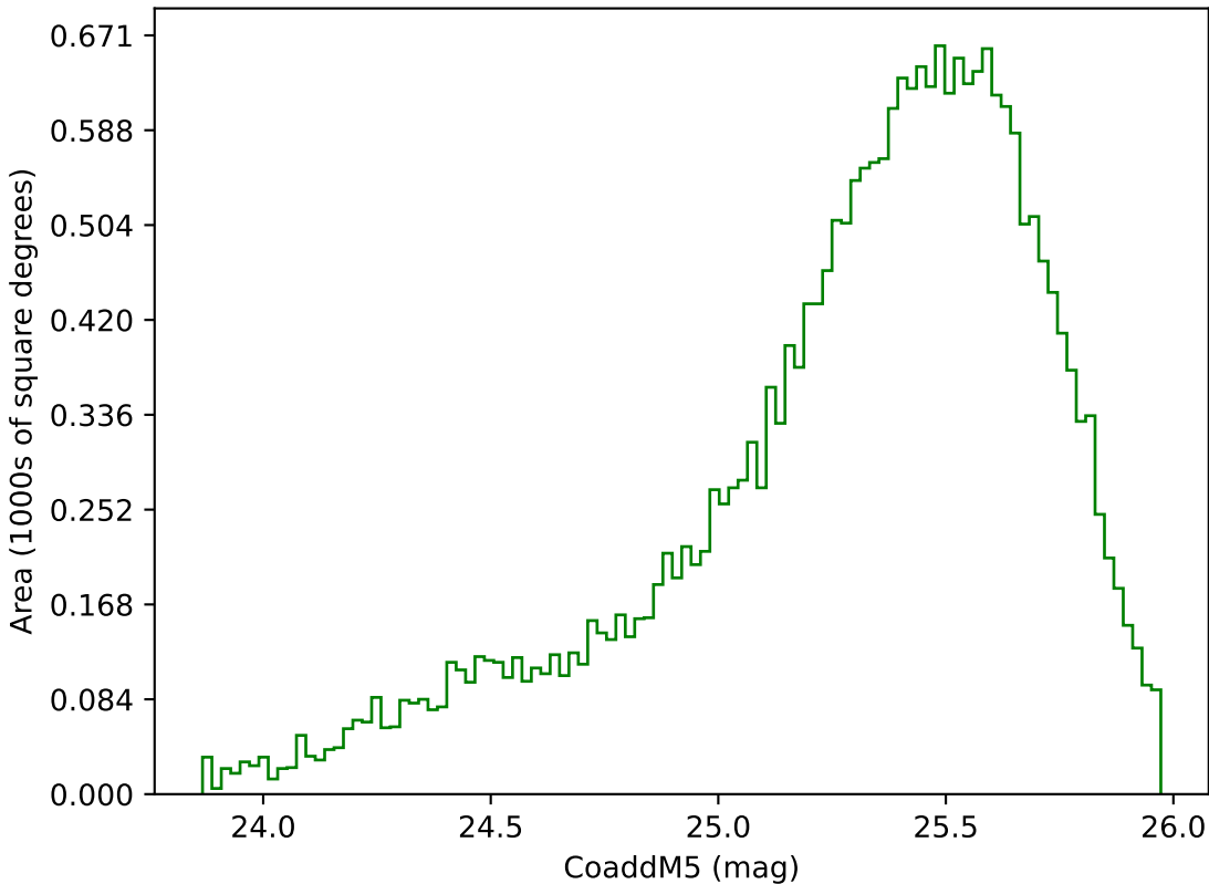
noroll_mjdp180_v3.4_10yrs Yr 3-4 g band: CoaddM5
