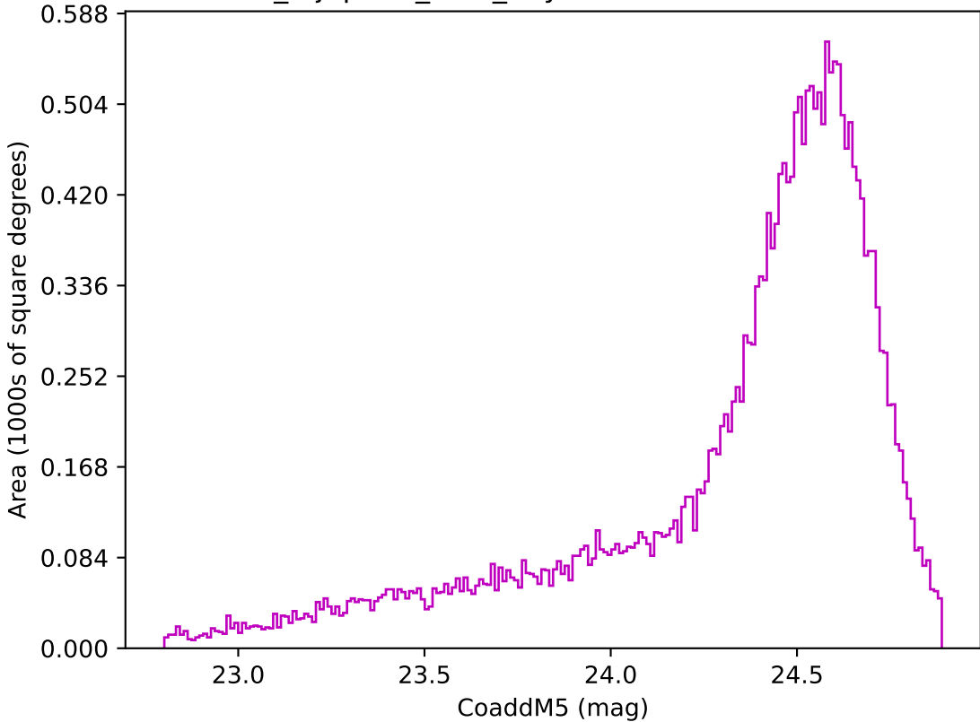
noroll_mjdp180_v3.4_10yrs Yr 1 z band: CoaddM5
