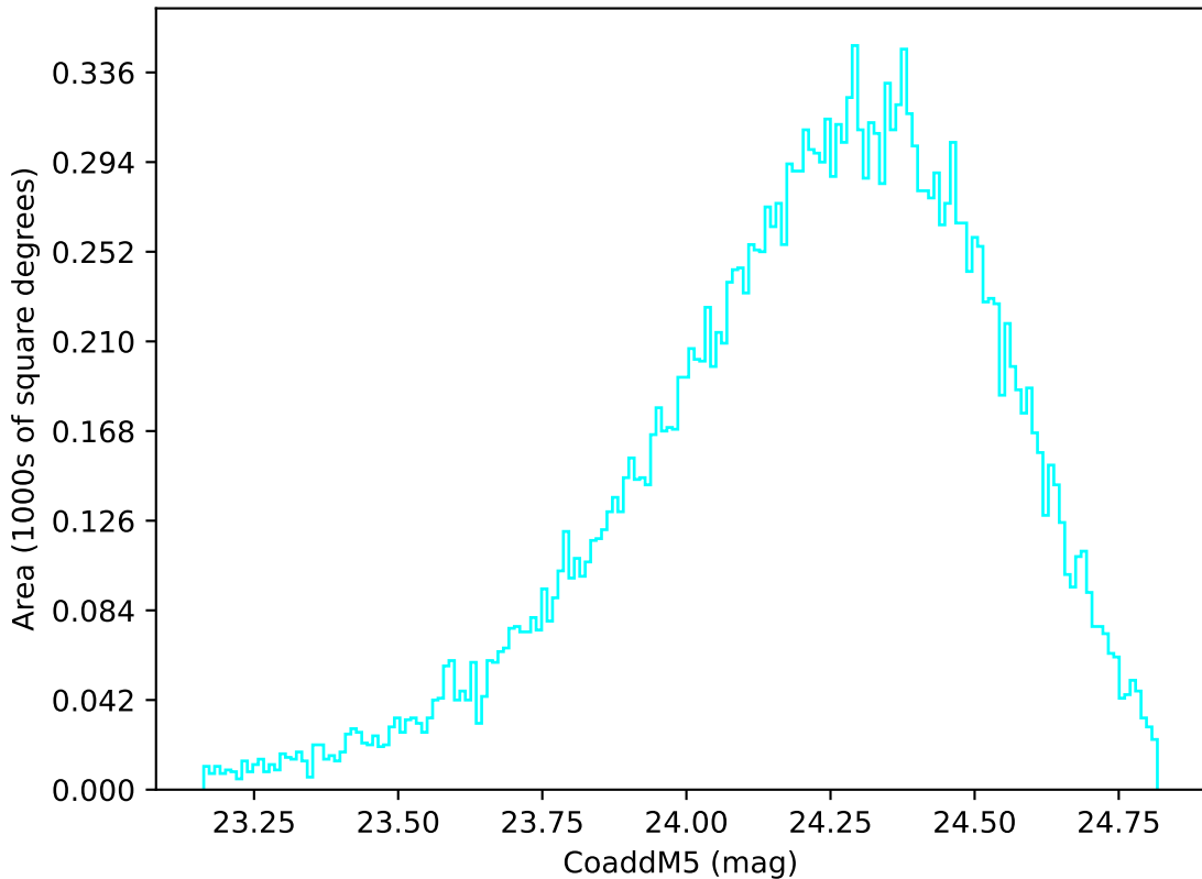
noroll_mjdp180_v3.4_10yrs Yr 1 u band: CoaddM5
