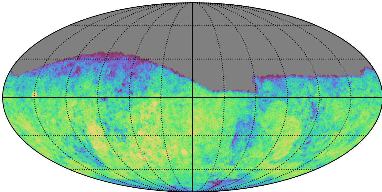
noroll_mjdp180_v3.4_10yrs Yr 1 g band: CoaddM5
