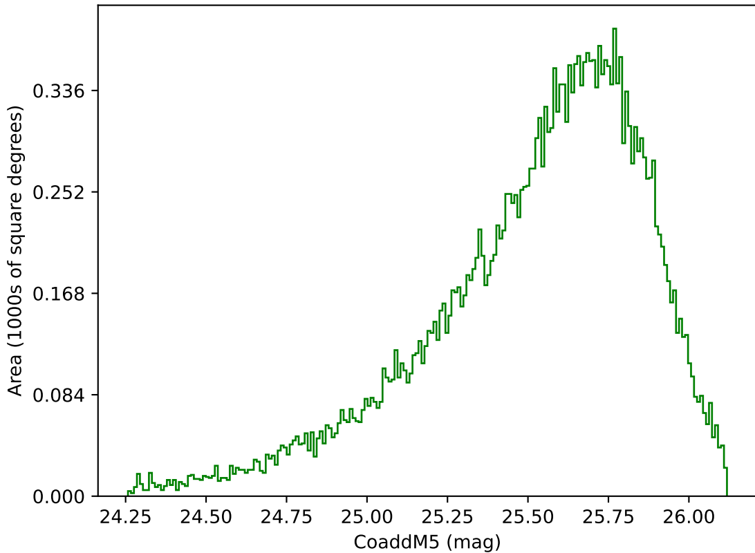
noroll_mjdp180_v3.4_10yrs Yr 1 g band: CoaddM5
