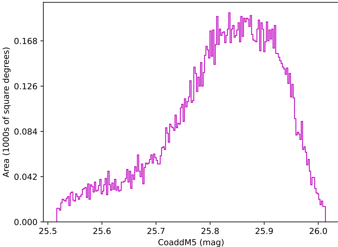
noroll_mjdp180_v3.4_10yrs WFD z band: CoaddM5
