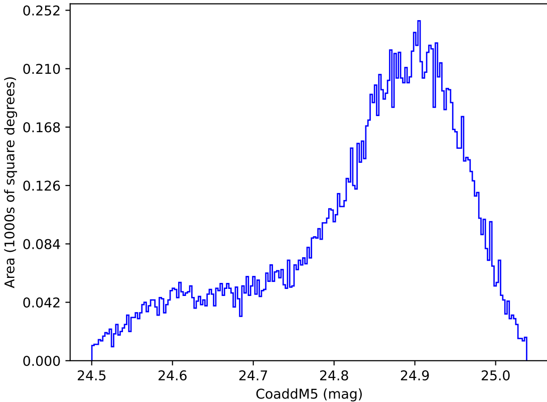
noroll_mjdp180_v3.4_10yrs WFD y band: CoaddM5
