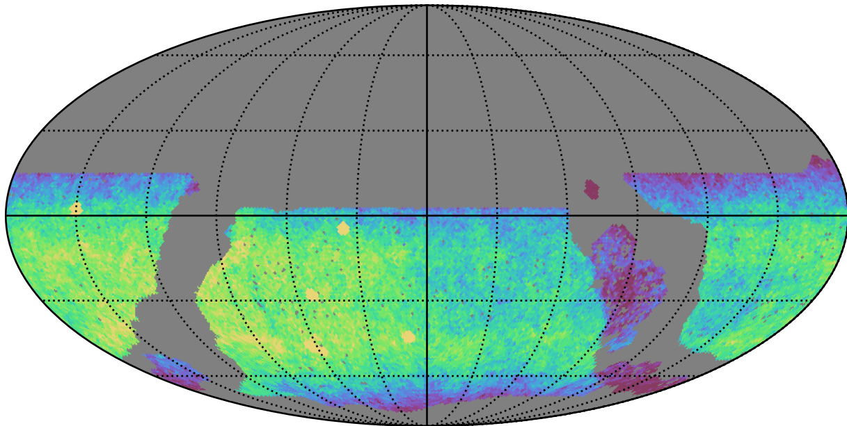
noroll_mjdp180_v3.4_10yrs WFD u band: CoaddM5
