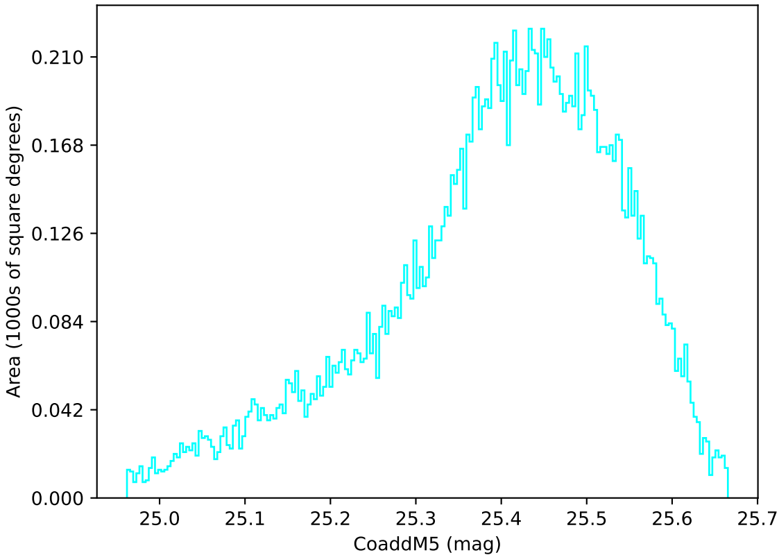
noroll_mjdp180_v3.4_10yrs WFD u band: CoaddM5
