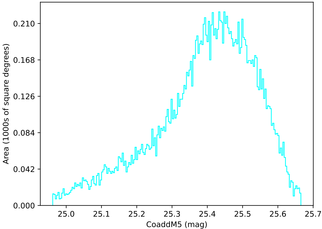
noroll_mjdp180_v3.4_10yrs WFD u band: CoaddM5
