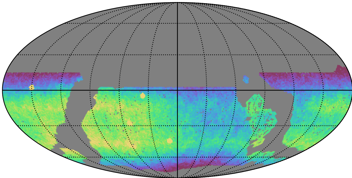
noroll_mjdp180_v3.4_10yrs WFD r band: CoaddM5
