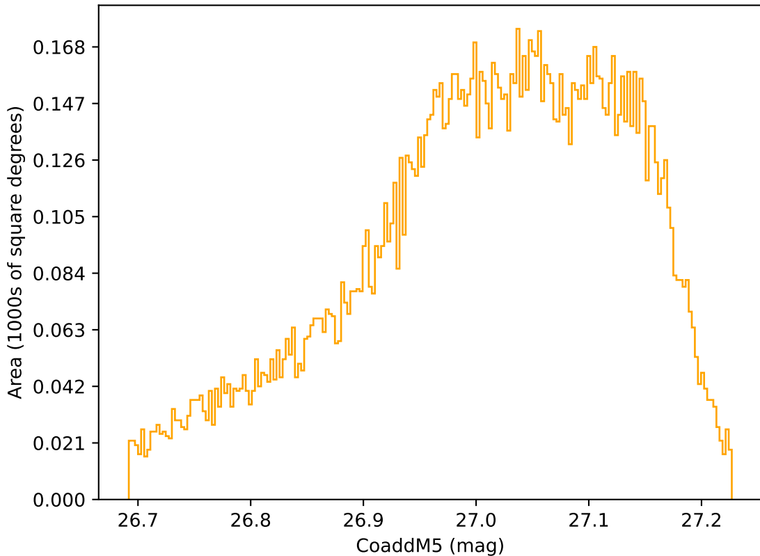
noroll_mjdp180_v3.4_10yrs WFD r band: CoaddM5
