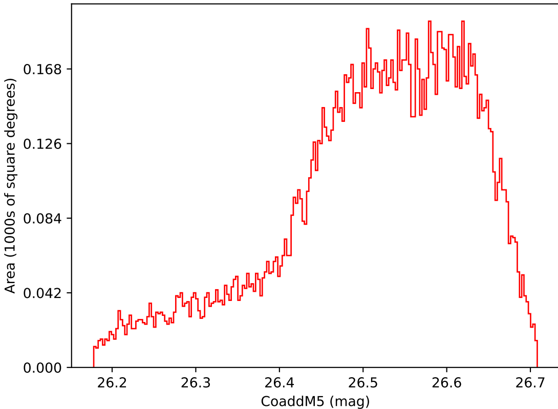
noroll_mjdp180_v3.4_10yrs WFD i band: CoaddM5
