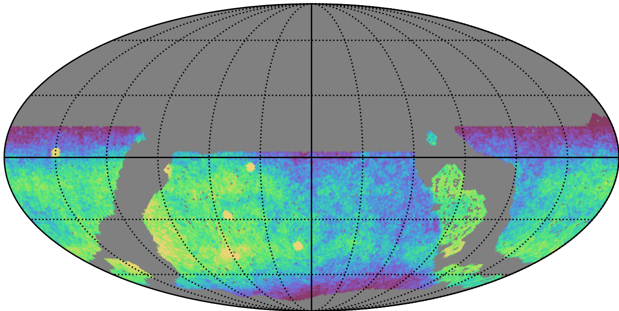
noroll_mjdp180_v3.4_10yrs WFD g band: CoaddM5
