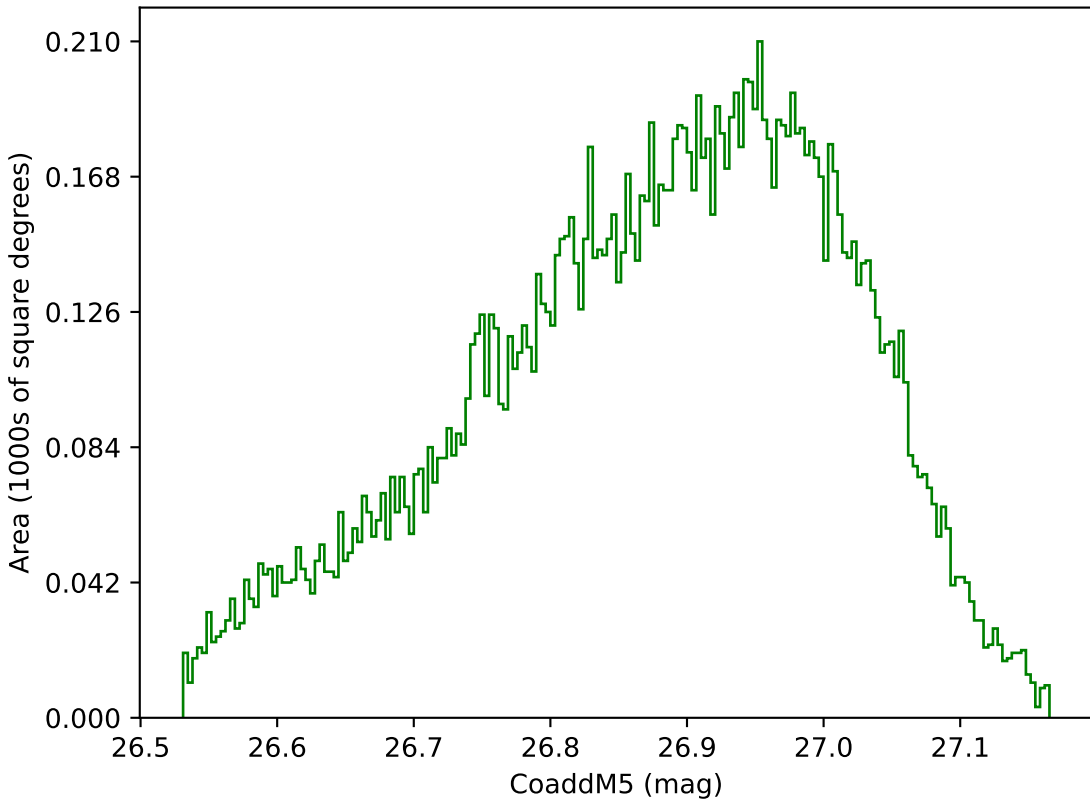
noroll_mjdp180_v3.4_10yrs WFD g band: CoaddM5
