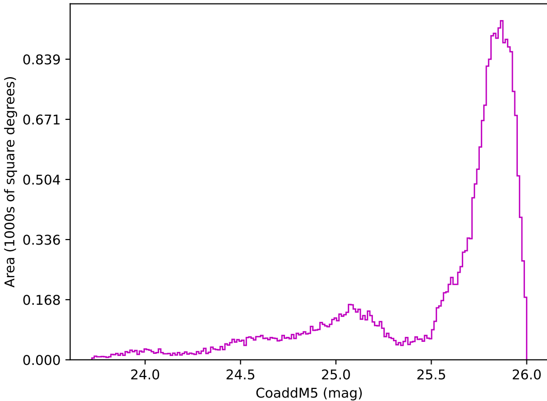
noroll_mjdp180_v3.4_10yrs All sky z band: CoaddM5
