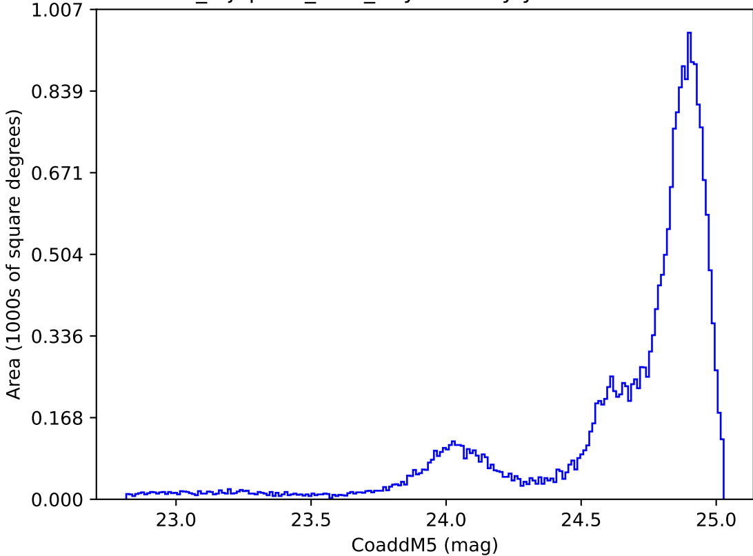
noroll_mjdp180_v3.4_10yrs All sky y band: CoaddM5
