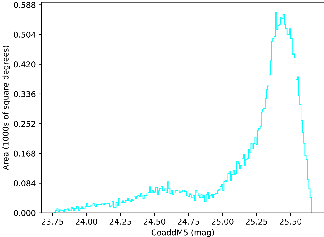
noroll_mjdp180_v3.4_10yrs All sky u band: CoaddM5
