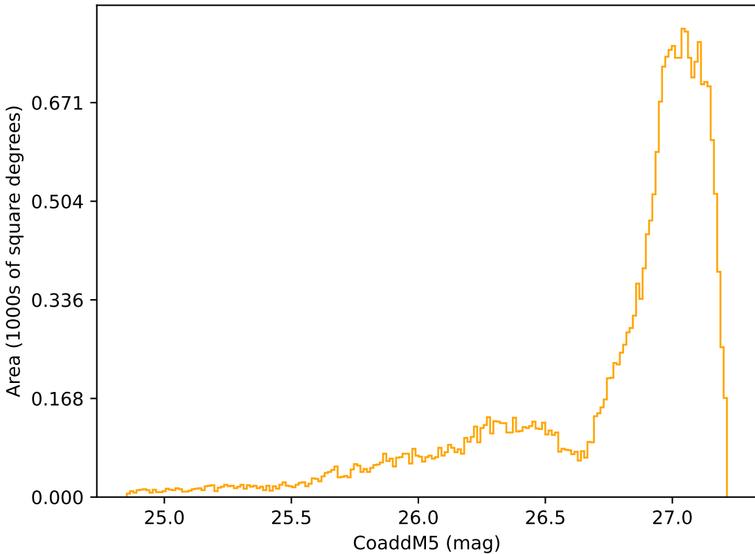
noroll_mjdp180_v3.4_10yrs All sky r band: CoaddM5
