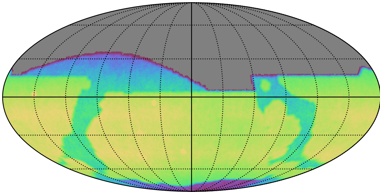
noroll_mjdp180_v3.4_10yrs All sky i band: CoaddM5
