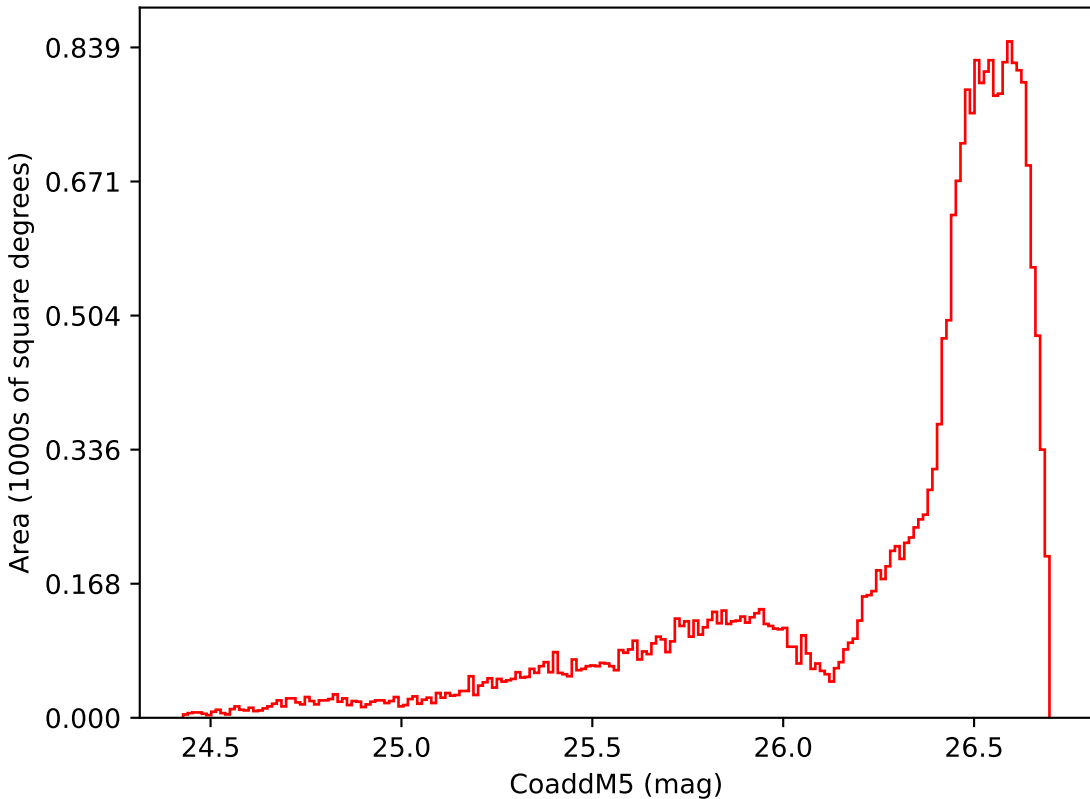
noroll_mjdp180_v3.4_10yrs All sky i band: CoaddM5
