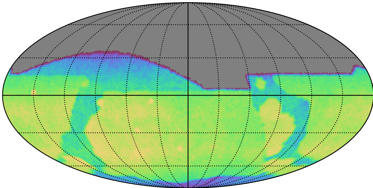
noroll_mjdp180_v3.4_10yrs All sky g band: CoaddM5
