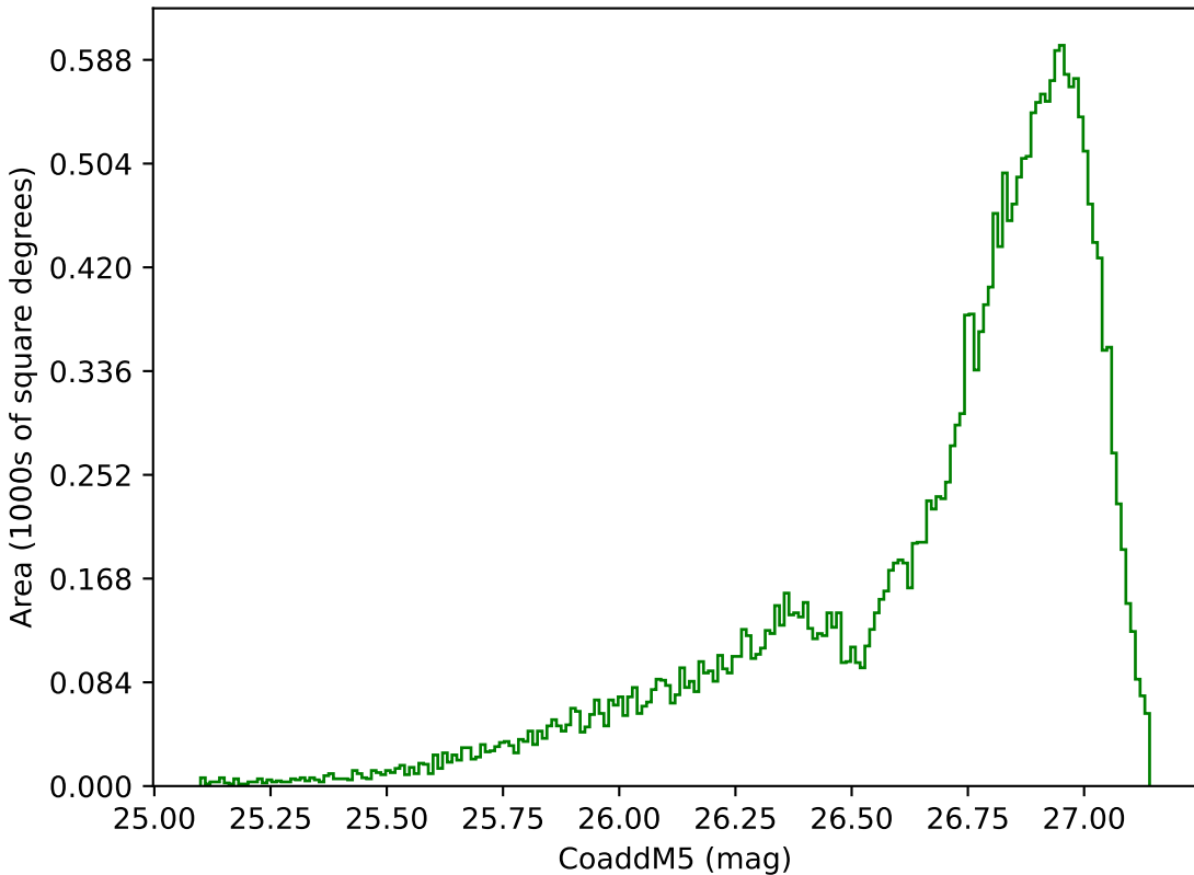
noroll_mjdp180_v3.4_10yrs All sky g band: CoaddM5
