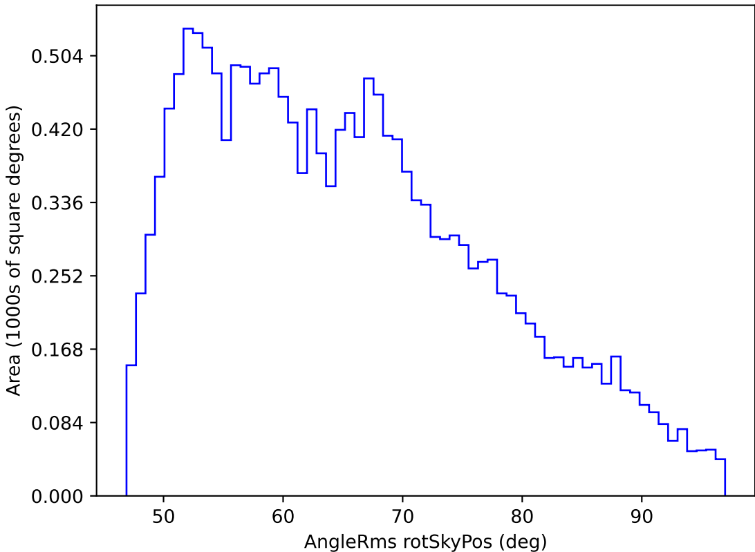
noroll_mjdp180_v3.4_10yrs WFD z band: AngleRms rotSkyPos
