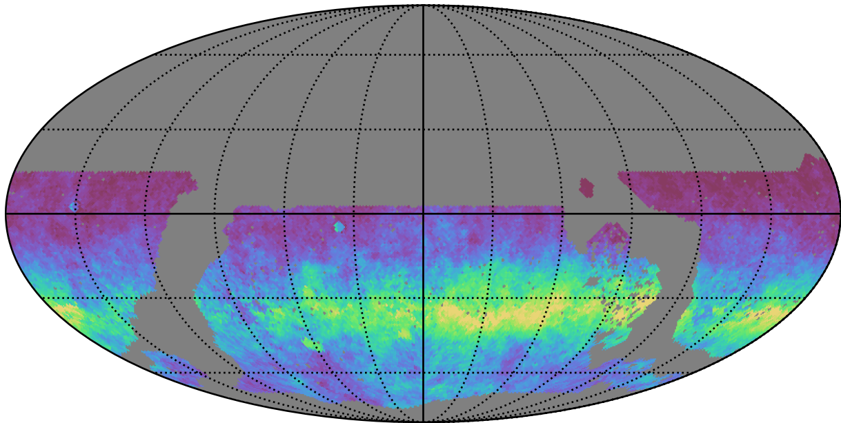
noroll_mjdp180_v3.4_10yrs WFD y band: AngleRms rotSkyPos
