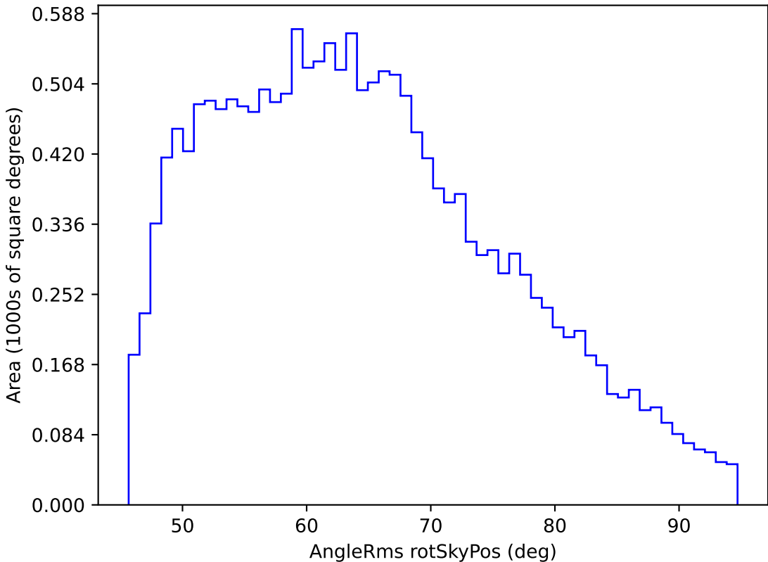
noroll_mjdp180_v3.4_10yrs WFD y band: AngleRms rotSkyPos
