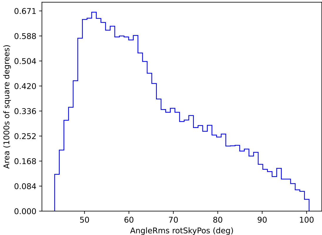
noroll_mjdp180_v3.4_10yrs WFD u band: AngleRms rotSkyPos
