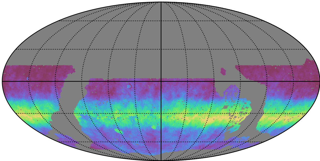
noroll_mjdp180_v3.4_10yrs WFD r band: AngleRms rotSkyPos
