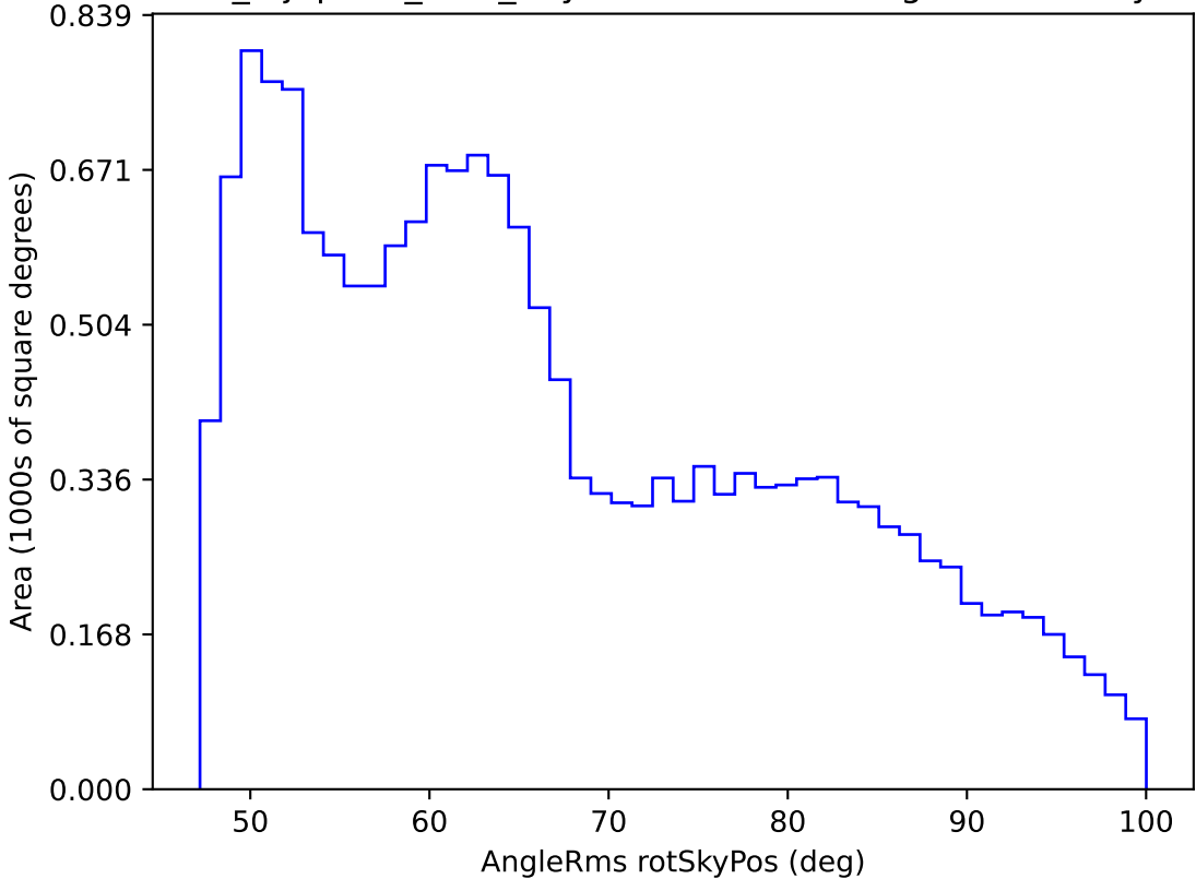
noroll_mjdp180_v3.4_10yrs WFD r band: AngleRms rotSkyPos
