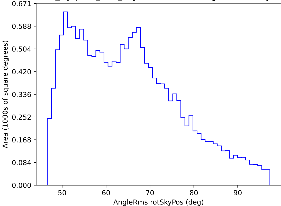
noroll_mjdp180_v3.4_10yrs WFD i band: AngleRms rotSkyPos
