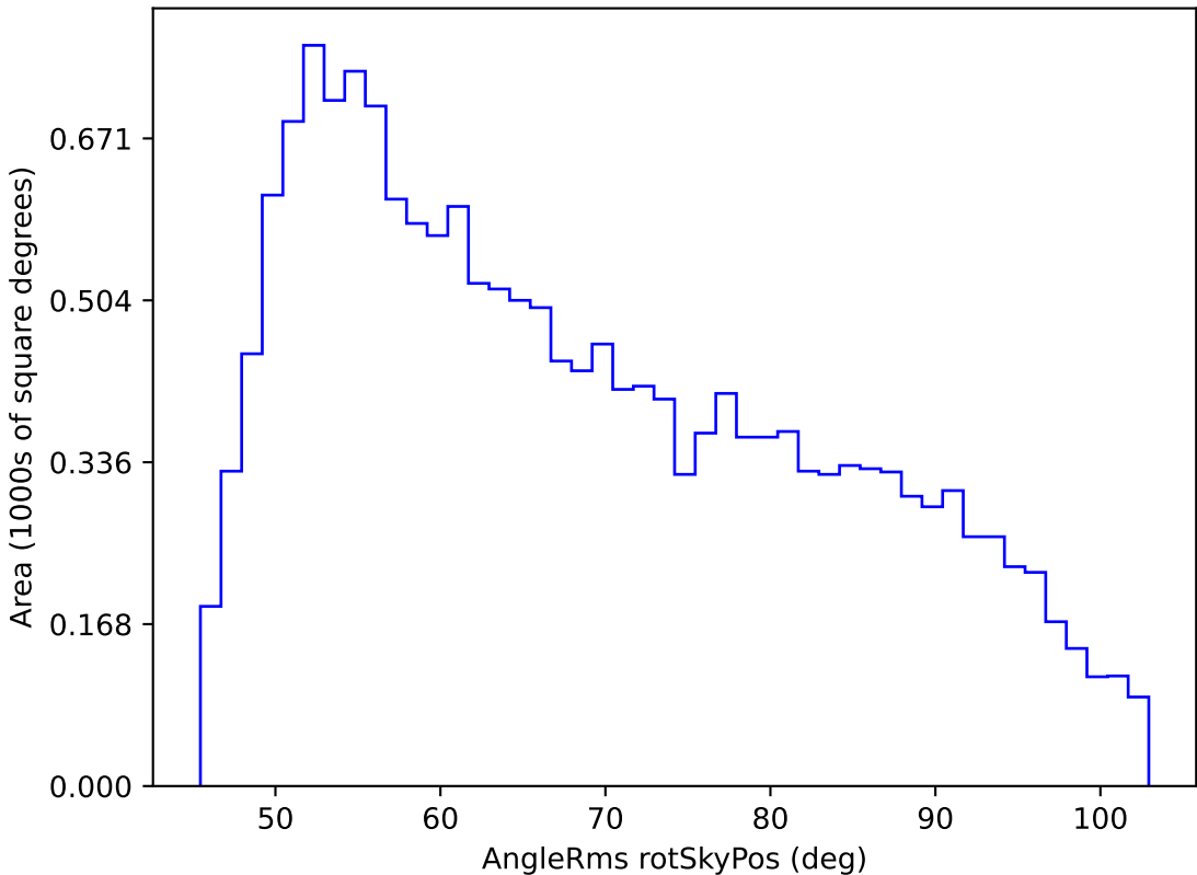
noroll_mjdp180_v3.4_10yrs WFD g band: AngleRms rotSkyPos
