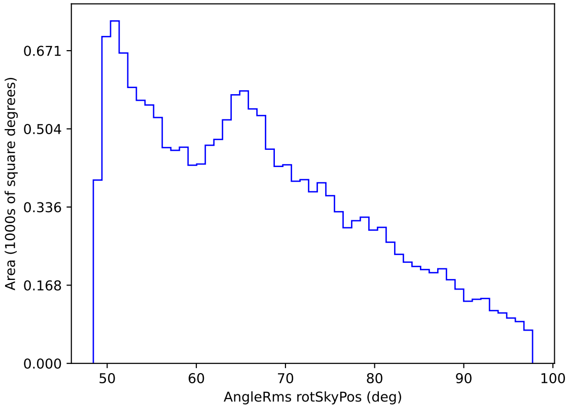
noroll_mjdp180_v3.4_10yrs WFD all bands: AngleRms rotSkyPos
