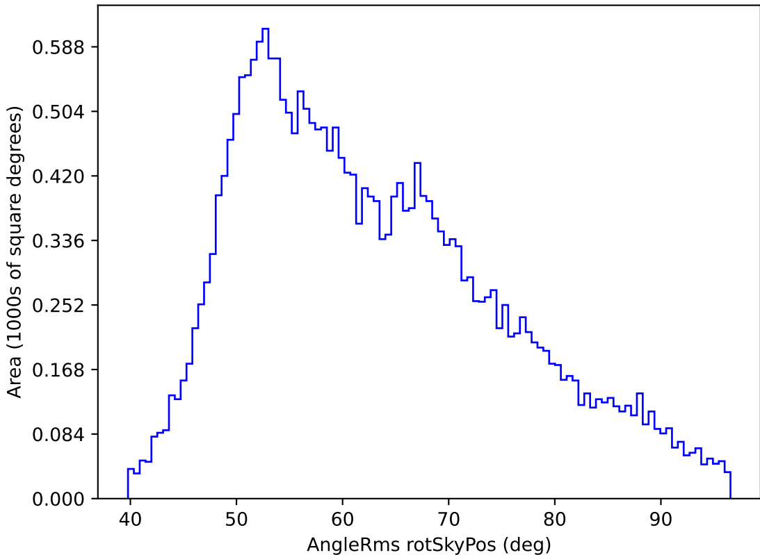
noroll_mjdp180_v3.4_10yrs All sky z band: AngleRms rotSkyPos
