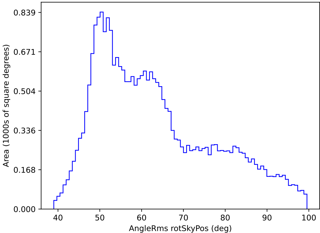
noroll_mjdp180_v3.4_10yrs All sky r band: AngleRms rotSkyPos
