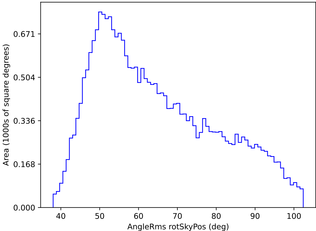
noroll_mjdp180_v3.4_10yrs All sky g band: AngleRms rotSkyPos
