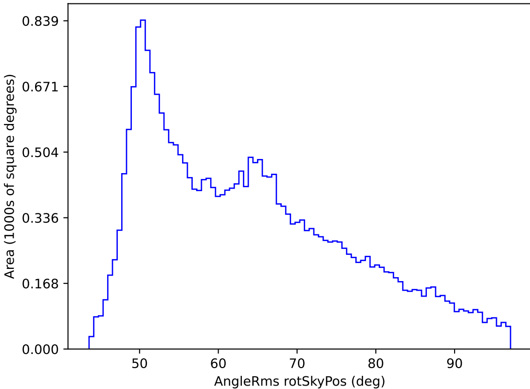
noroll_mjdp180_v3.4_10yrs All sky all bands: AngleRms rotSkyPos
