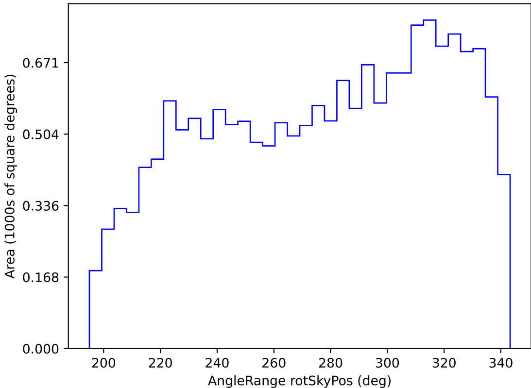
noroll_mjdp180_v3.4_10yrs WFD z band: AngleRange rotSkyPos
