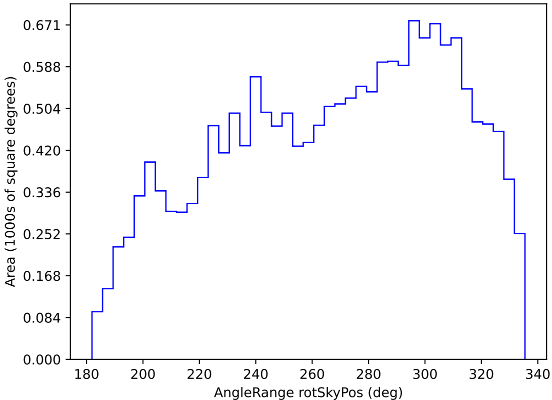
noroll_mjdp180_v3.4_10yrs WFD y band: AngleRange rotSkyPos
