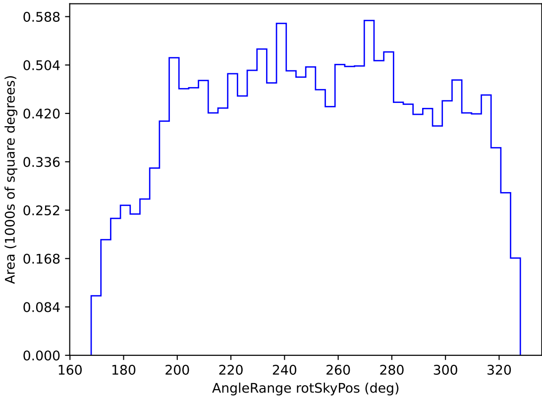
noroll_mjdp180_v3.4_10yrs WFD u band: AngleRange rotSkyPos
