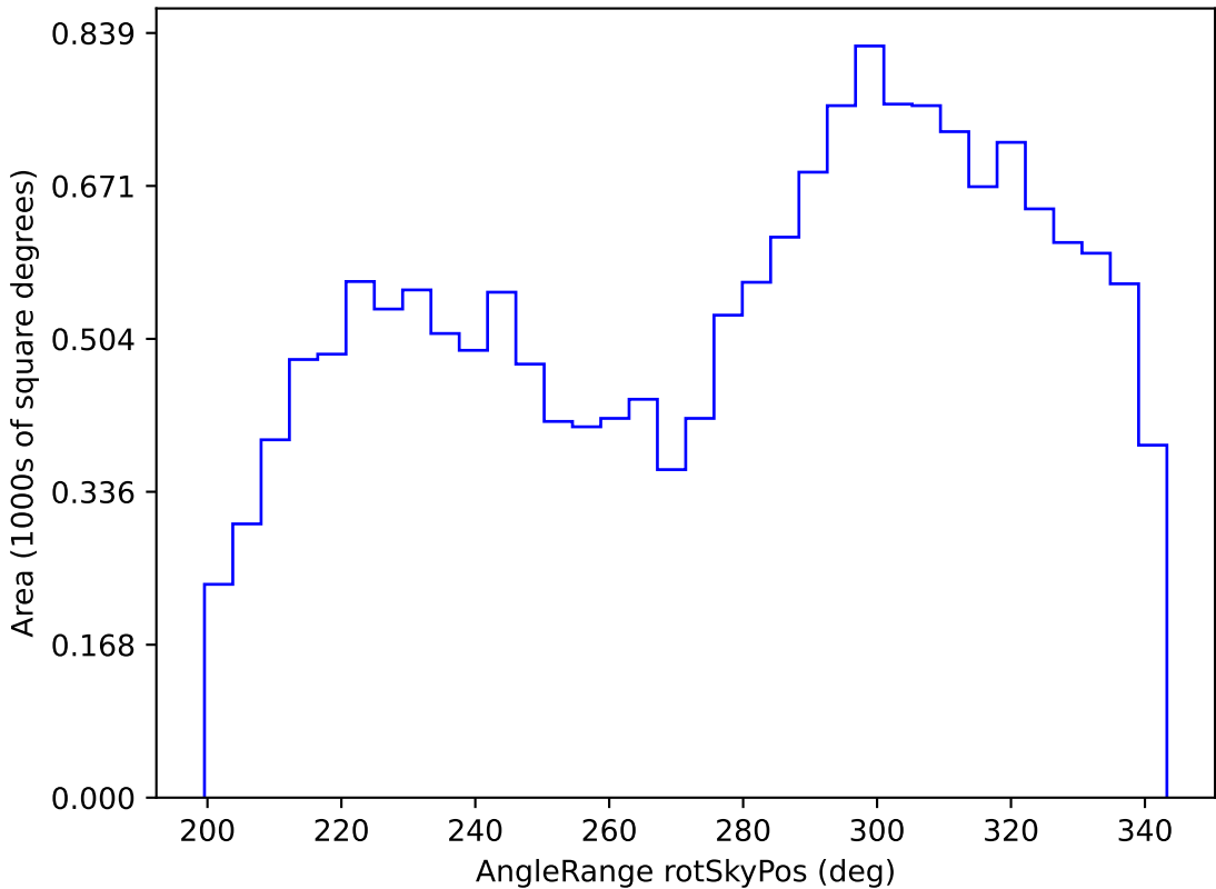
noroll_mjdp180_v3.4_10yrs WFD r band: AngleRange rotSkyPos
