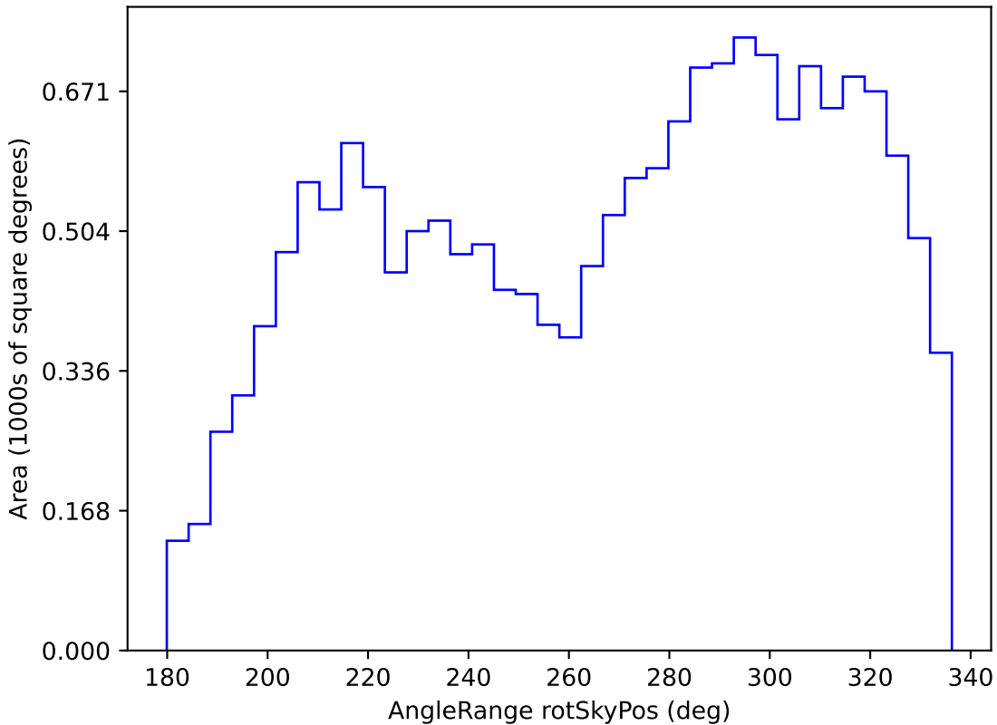
noroll_mjdp180_v3.4_10yrs WFD g band: AngleRange rotSkyPos
