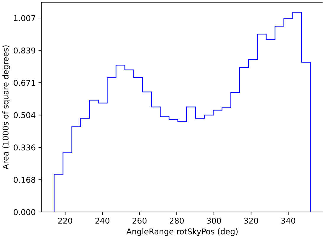
noroll_mjdp180_v3.4_10yrs WFD all bands: AngleRange rotSkyPos
