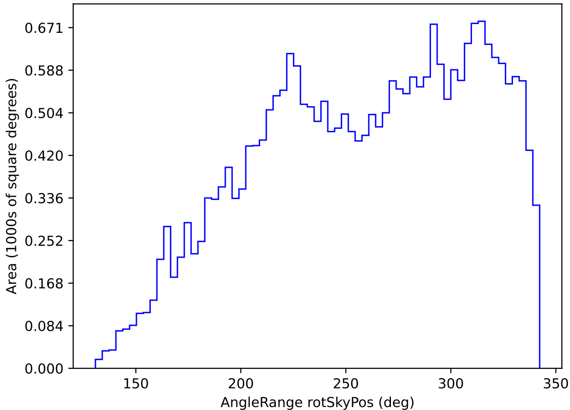
noroll_mjdp180_v3.4_10yrs All sky z band: AngleRange rotSkyPos
