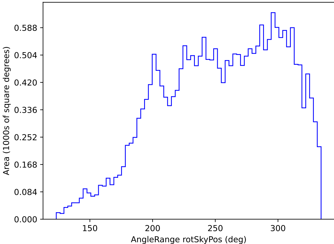
noroll_mjdp180_v3.4_10yrs All sky y band: AngleRange rotSkyPos
