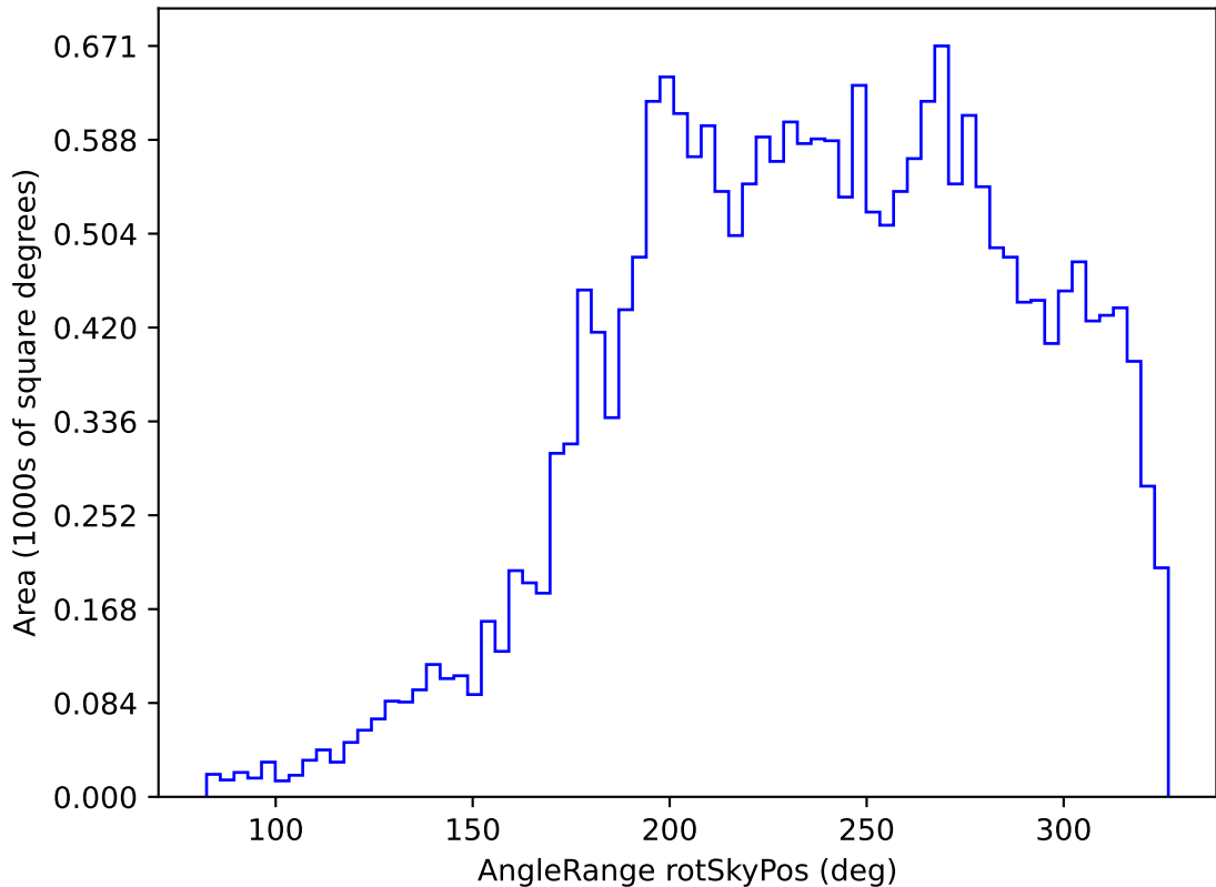
noroll_mjdp180_v3.4_10yrs All sky u band: AngleRange rotSkyPos
