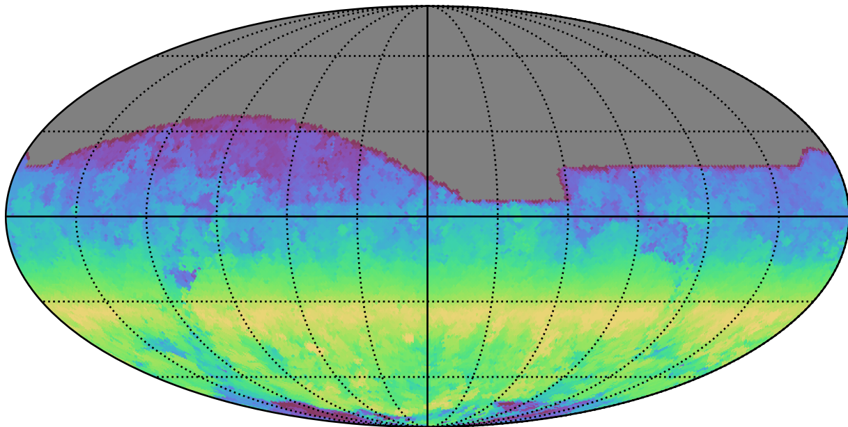
noroll_mjdp180_v3.4_10yrs All sky r band: AngleRange rotSkyPos
