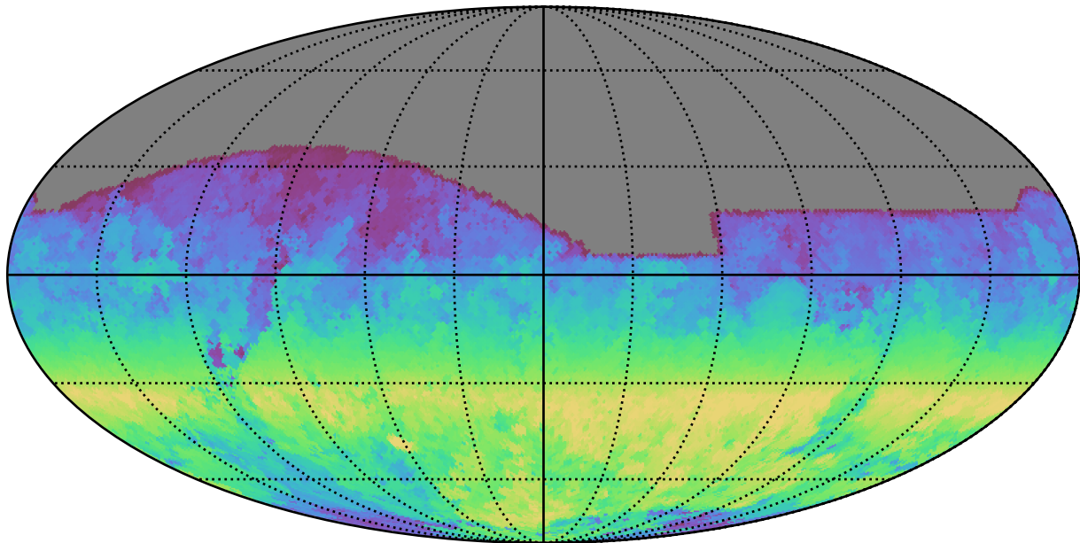
noroll_mjdp180_v3.4_10yrs All sky i band: AngleRange rotSkyPos
