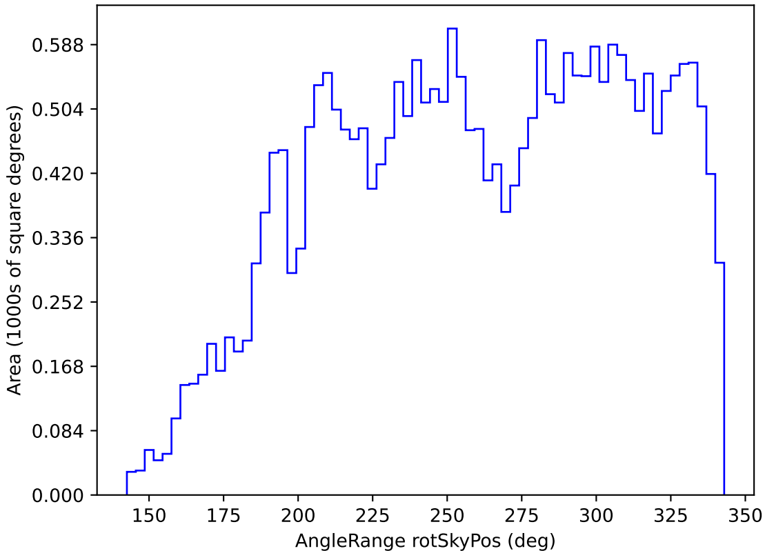
noroll_mjdp180_v3.4_10yrs All sky i band: AngleRange rotSkyPos
